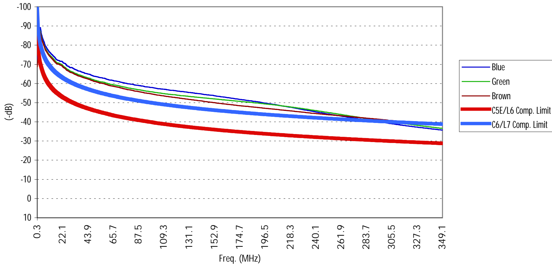
DataGate 6 Component Power Sum ACR, All Pairs
