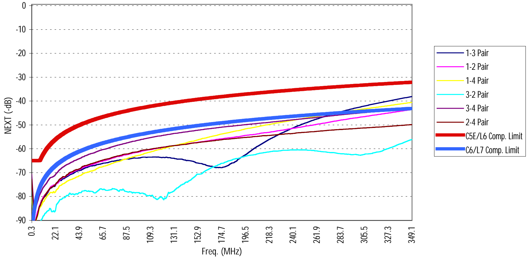
DataGate 6 Component NeXT, All Pairs
